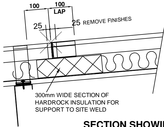
SECTION SHOWING SHEET LAP
