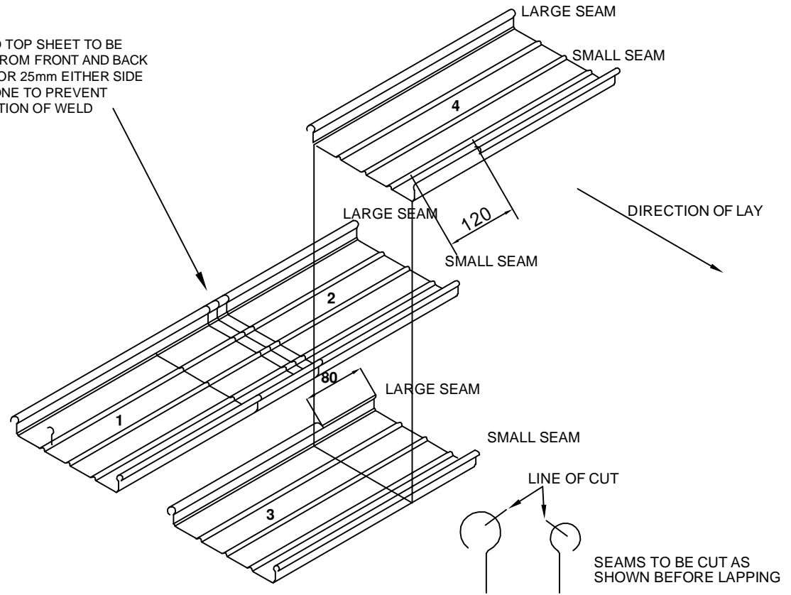
EXPLODED ISOMETRIC VIEW OF LAP DETAIL
