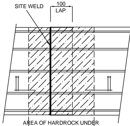
PLAN VIEW OF SITE WELDED LAP
